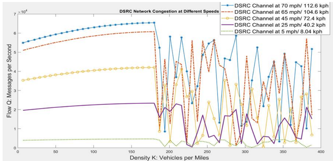
Figure 5.5. Channel Congestion when Density is more than 187 vehicles (45 mph)
